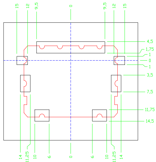
Recommended resist pattern
